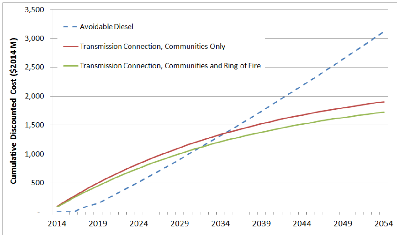
Figure 7: Transmission Connection Breaks Even in 20-25 Years versus Diesel Generation
