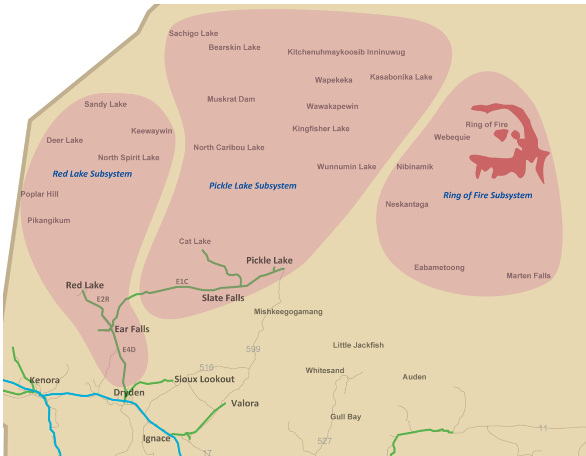
Figure 13: Community Subsystems
