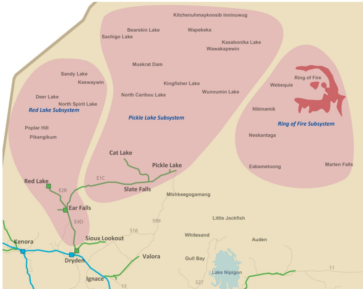
Figure 3: Community Subsystems
